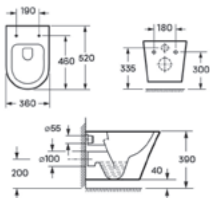
CLEMENT FALI RIMLESS WC
